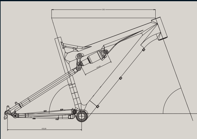
Engineering Drawing
